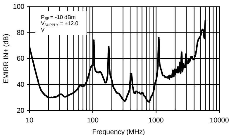
Figure 1. OPA211 EMIRR IN+ vs Frequency
